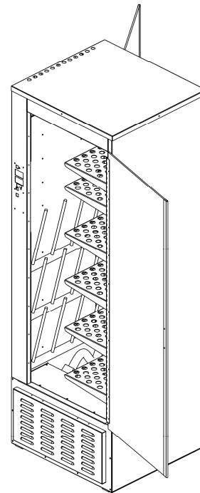
Model 136 with Bag & Bottle Rack Option
